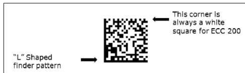
Figure 5.6.2-1. GS1 DataMatrix symbol
