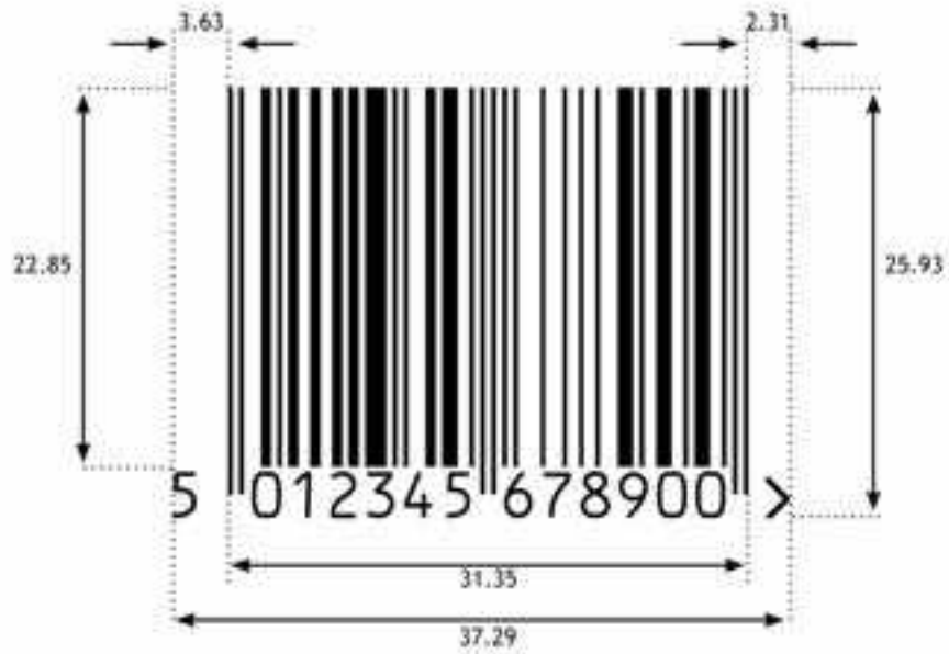
Figure 5.2.6.6-1. EAN-13 barcode
